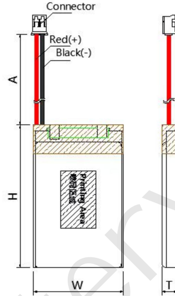
Drawing Of Battery Pack
