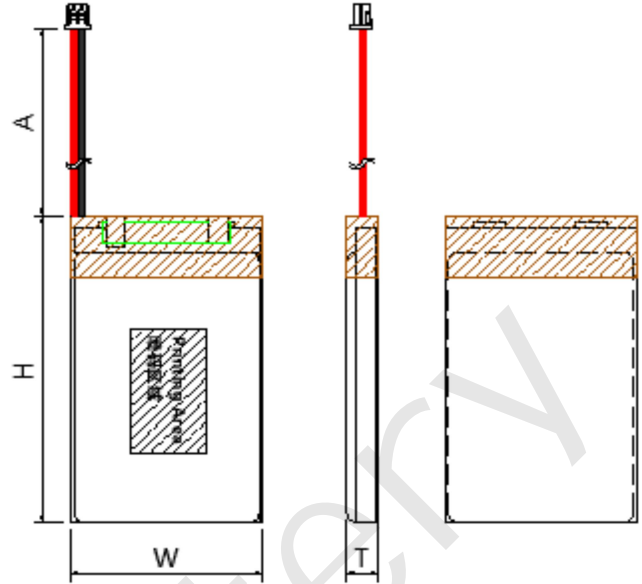
Drawing Of Battery Pack
