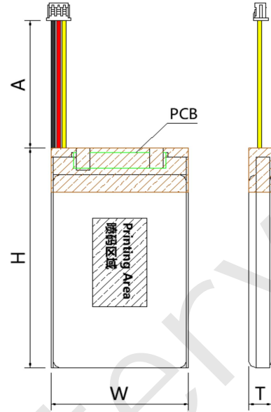
Drawing Of Battery Pack
