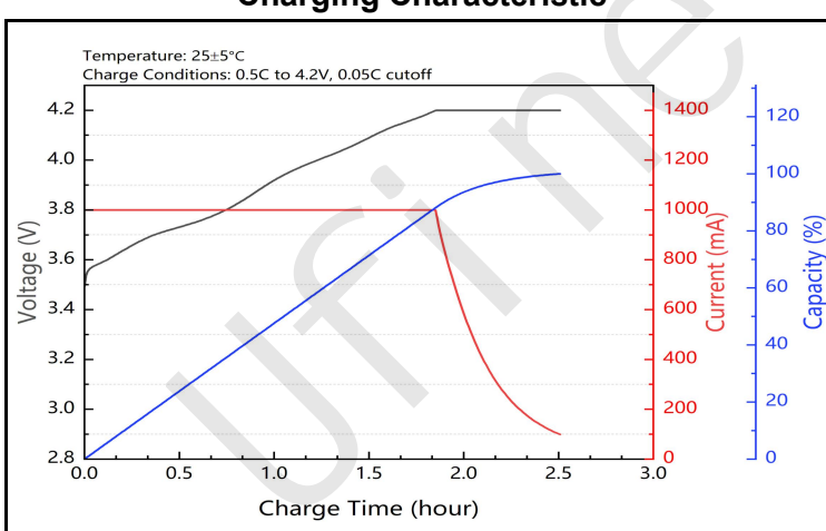
Charging Characteristic
