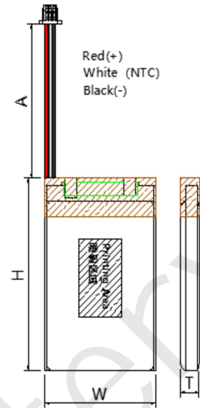
Drawing Of Battery Pack
