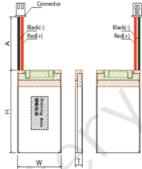
Drawing Of Battery Pack
