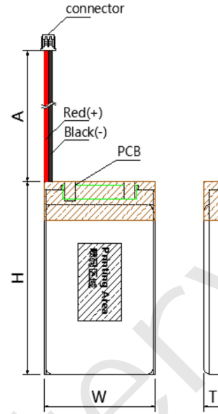
Drawing Of Battery Pack
