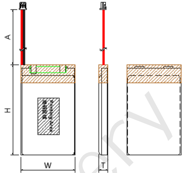
Drawing Of Battery Pack
