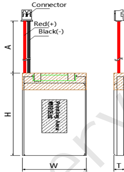
Drawing Of Battery Pack
