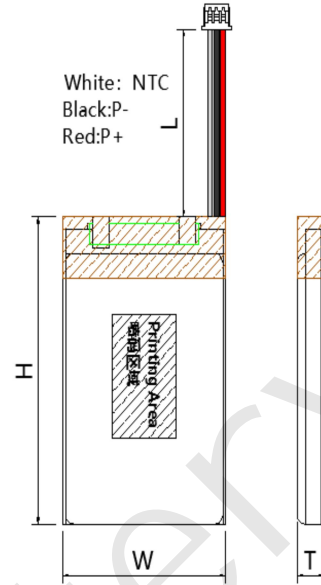
Drawing Of Battery Pack
