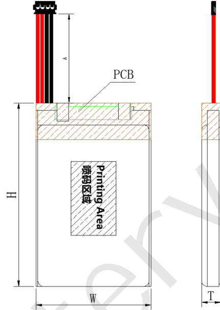
Drawing Of Battery Pack
