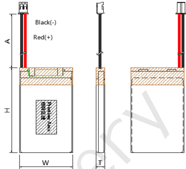
Drawing Of Battery Pack
