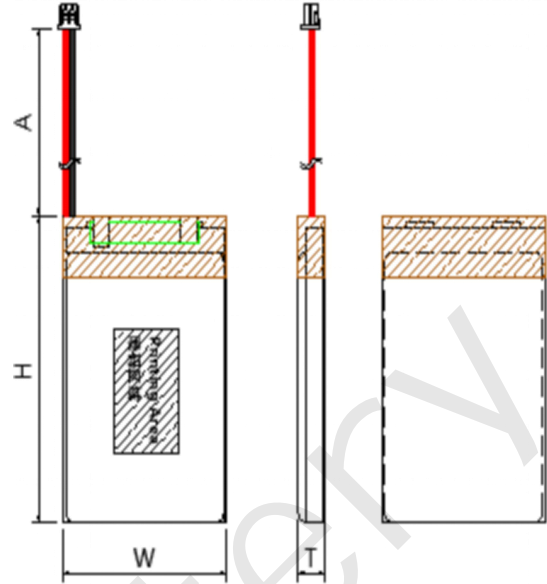
Drawing Of Battery Pack
